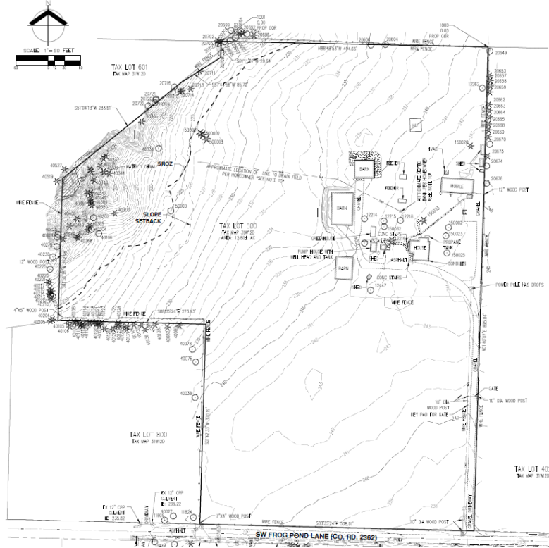
Existing Conditions
