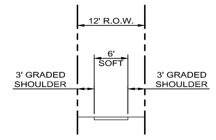
R NATURE PATHWAY NTS
