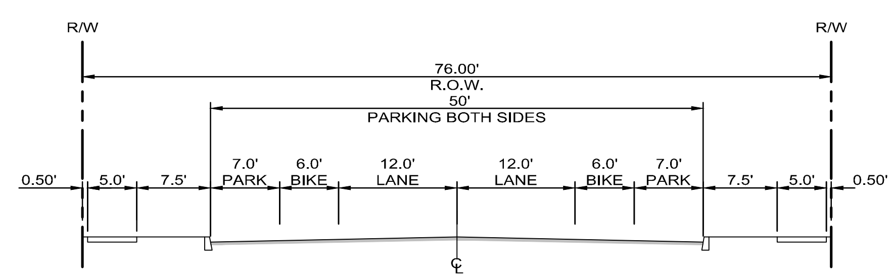
E MINOR COLLECTOR NTS
