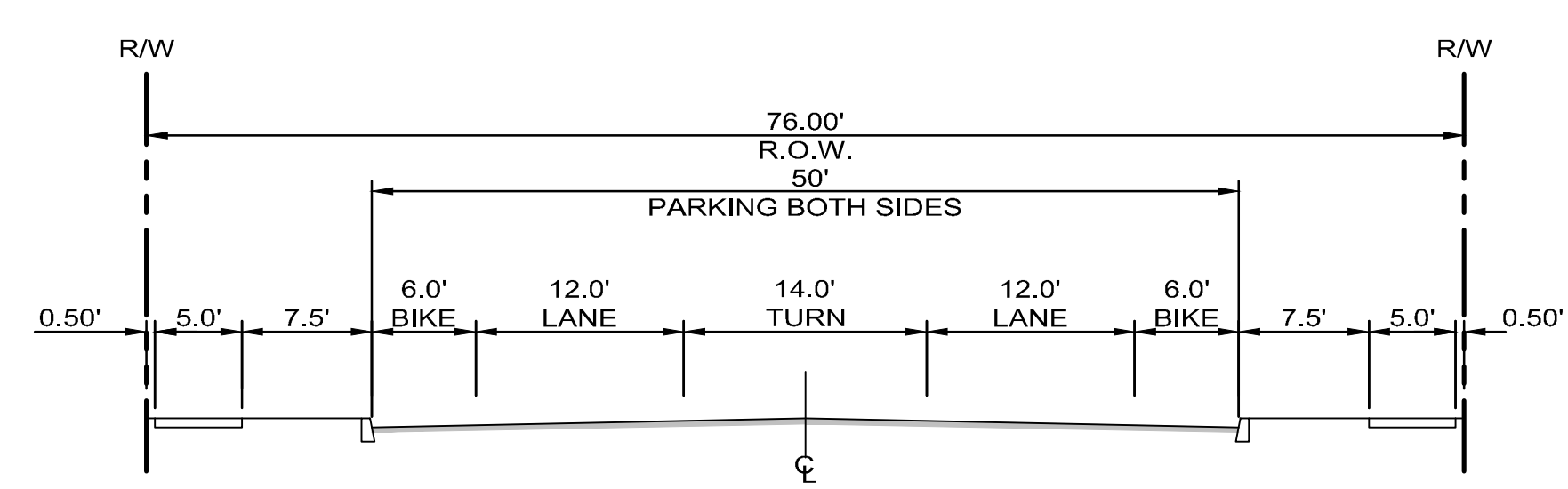
E1 MINOR COLLECTOR W/LEFT TURN POCKET NTS
