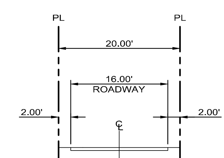
O PRIVATE LANE NTS
