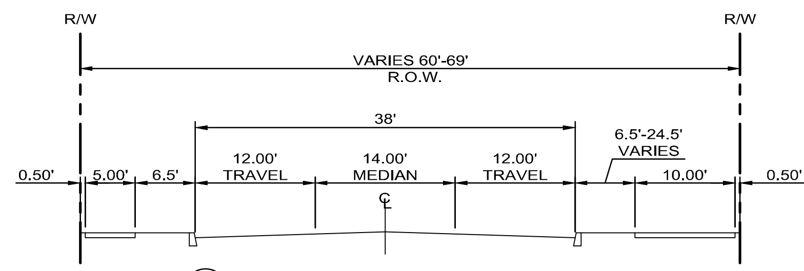
P MINOR ARTERIAL NTS
