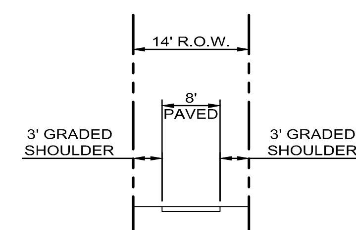
S MINOR PATHWAY NTS
