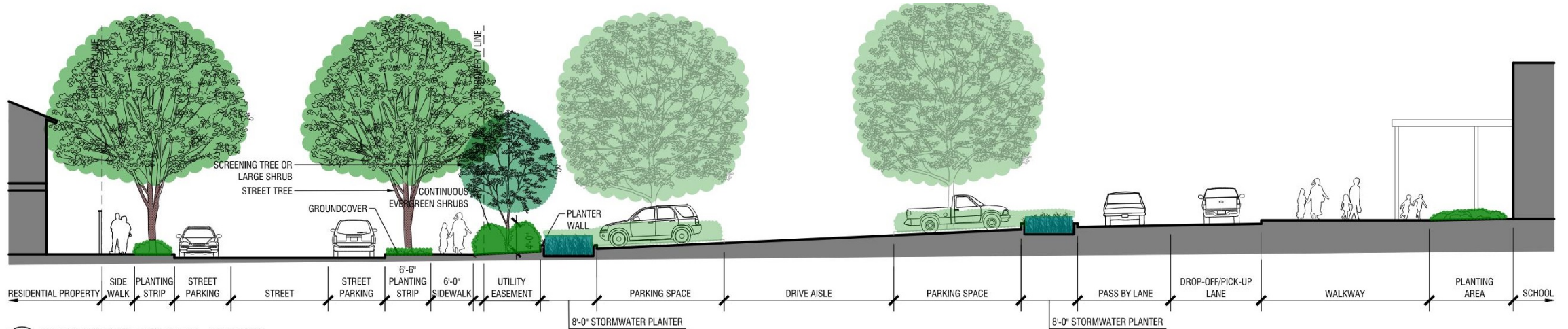
2 SHERMAN RIGHT OF WAY - SECTION SCALE: 1" = 10'-0"
